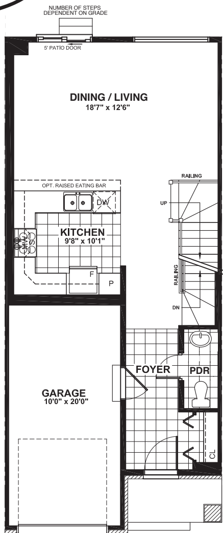
GROUND FLOOR 622 SQ. FT.
